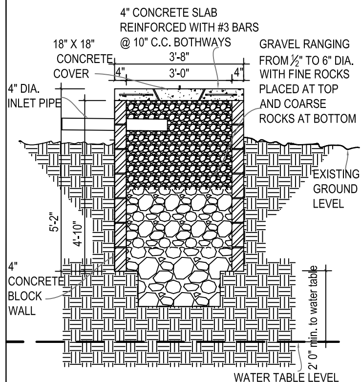
SECTION THRU SOAKAWAY SCALE: 3/8" = 1' 0"
